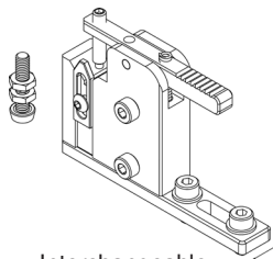
Interchangeable clamp inserts
